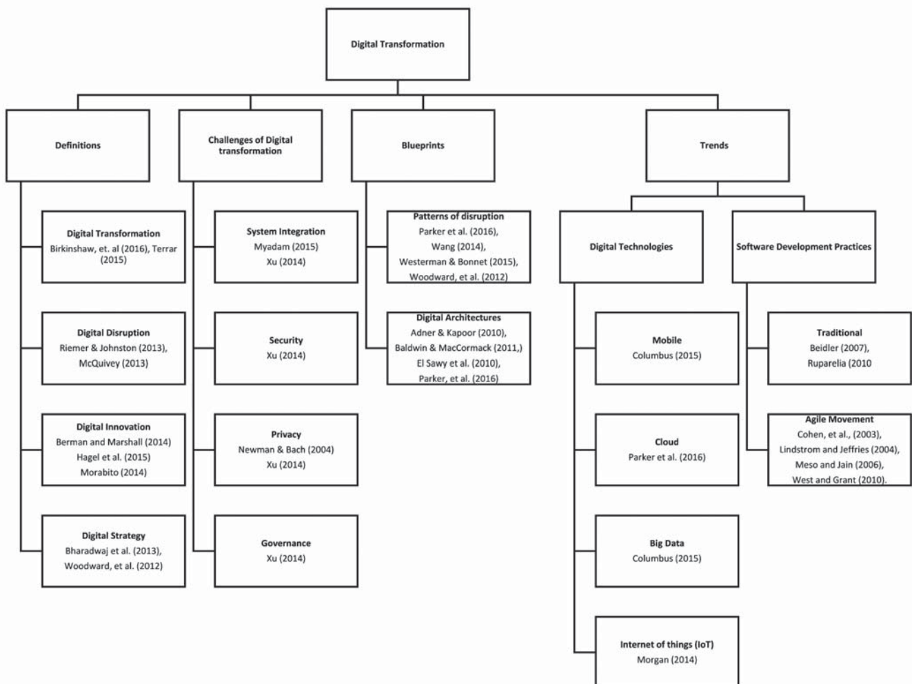
Figure 2: Literature map
